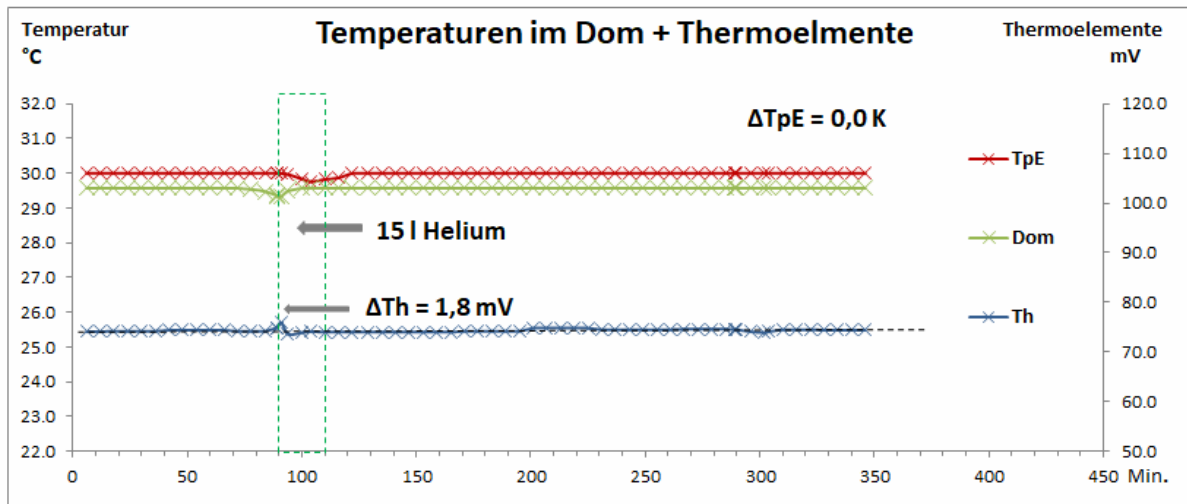
Abb. 6: Helium-Experiment Nr. 3: Endkonzentration 13 Vol.-% Helium
