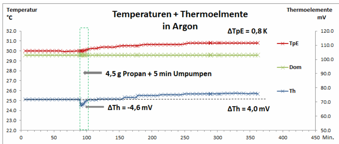
Abb. 3a: Propan-Experiment Nr. 6: Endkonzentration 2,0 Vol.-% Propan.
